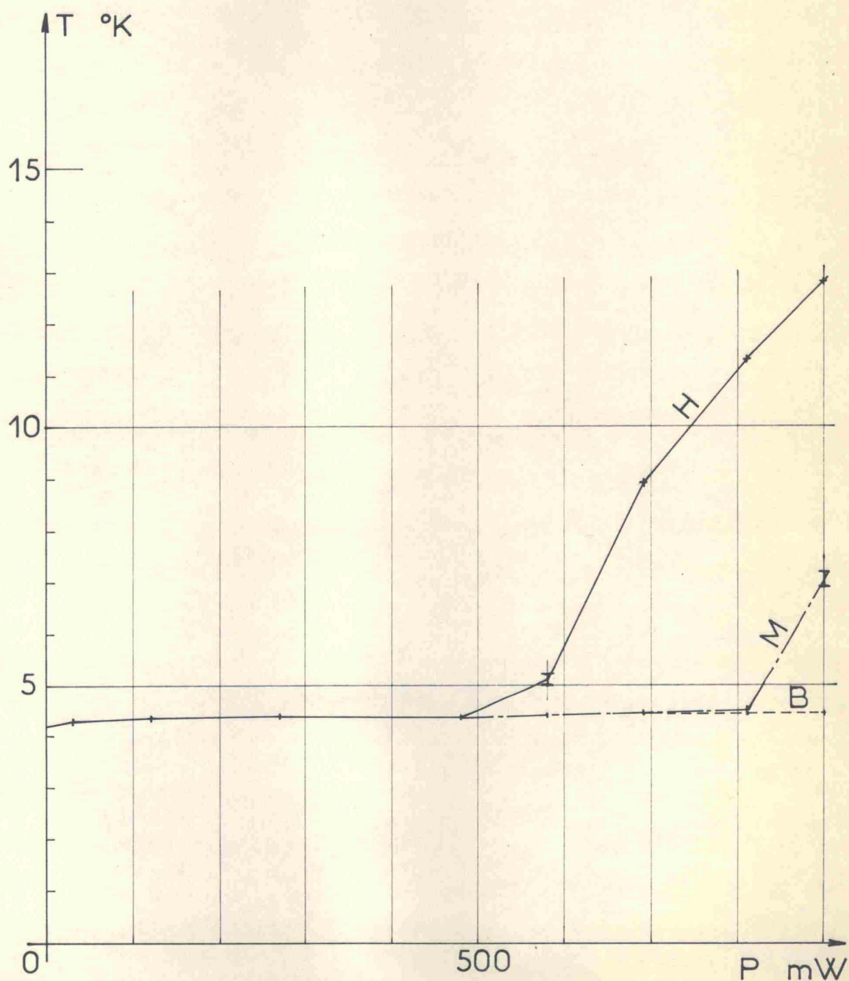
FIG.2 Normal helium T = 4.2 \text{ K} ; P = 760 \text{ mm Hg} Depth of immersion : 20 cm
